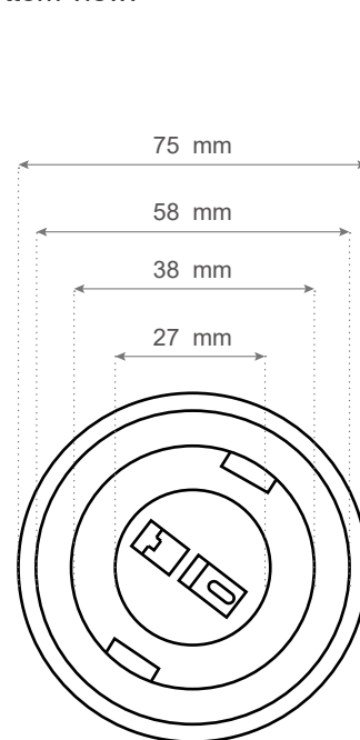
Bottom view:
