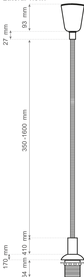
Lateral view:
