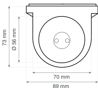
Top and bottom view:
