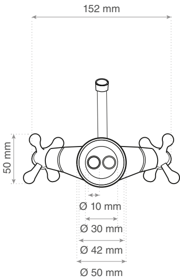
Bottom view:
