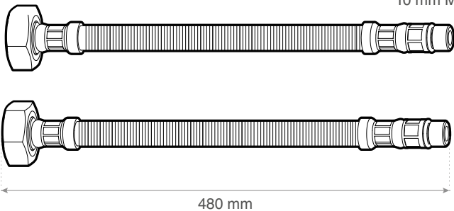
3/8" Female (12-17mm)
