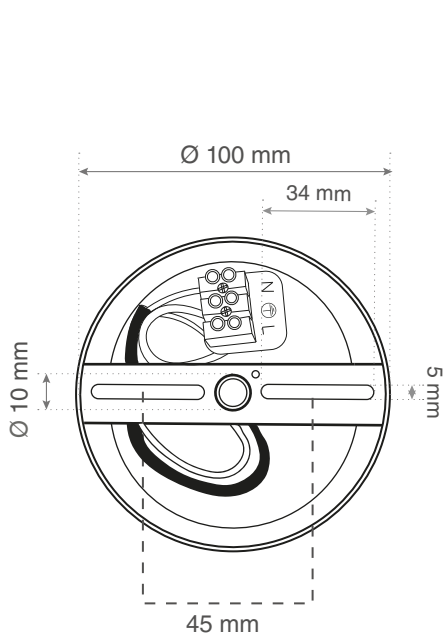
Bottom view:
