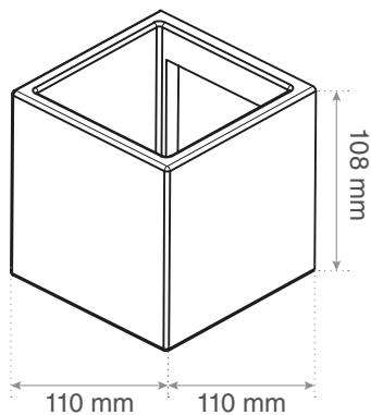
Perspective view:
